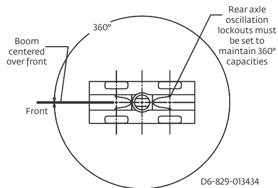
Diagram for lifting on tires
