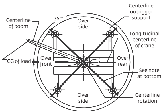
Diagram for lifting on outriggers
